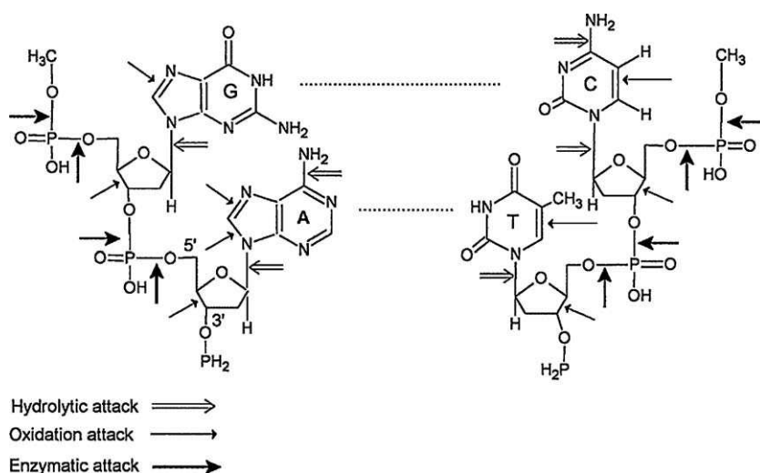
Fig. 2. Oxidation, hydrolytic and enzymatic attacks associated with DNA degradation. Redrawn with modifications from [20]. A: adenine, G: guanine, C: cytosine, T: thymine.
